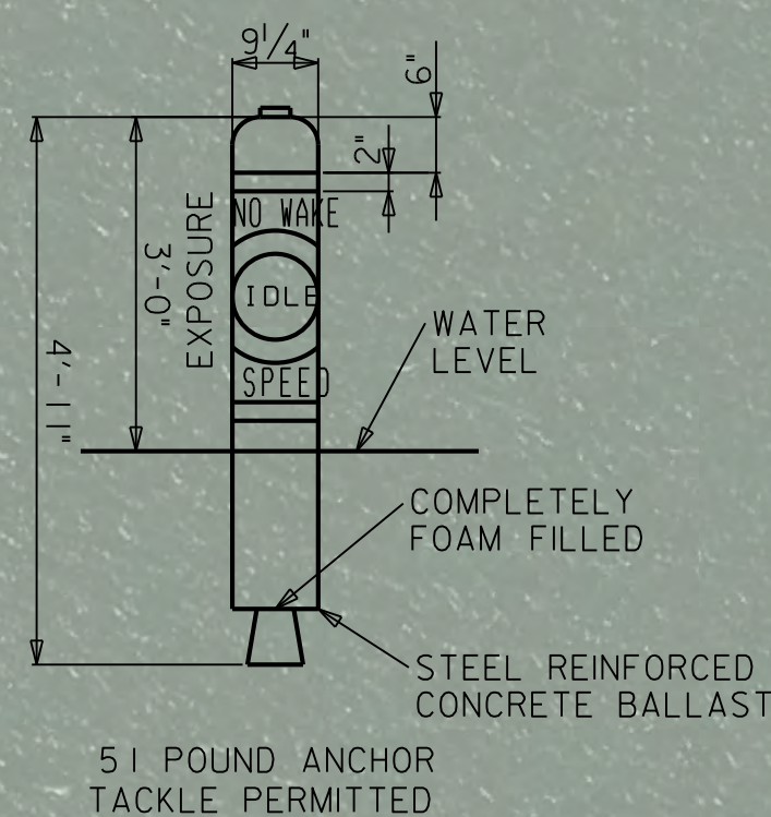
RESTRICTED AREA BUOY (*NO WAKE*) (6 REQUIRED - ROADWAY ITEM)
